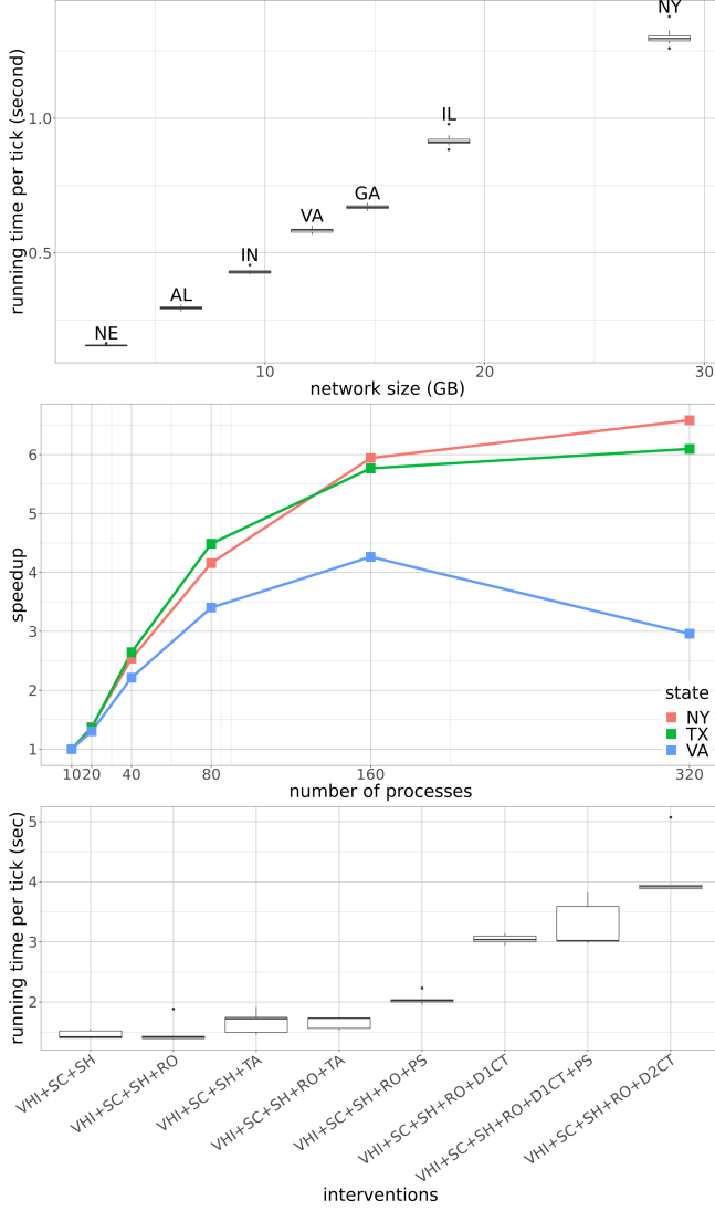
Figure 7. (top) Running time of EpiHiper on networks of different sizes given 40 processing units. (middle) As the number of processing units increase, the corresponding improvement in the performance of the simulations illustrates the strong scaling results of EpiHiper. Beyond some point, which varies with the problem size, the benefit of using more resources starts to diminish. (bottom) Running time of EpiHiper varies with different interventions in the simulation. Simulations with more interventions, or with more complex interventions, take more time.
